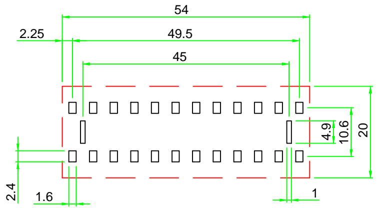
( PCB LAYOUT )
